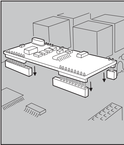
AM-3 SOCKET MODEM INSTALLATION
